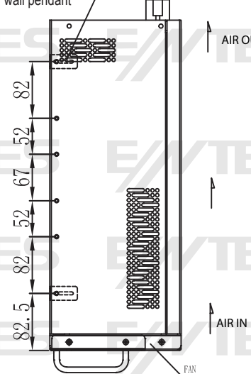
4-M4*8 Screw (Side) Fixed wall pendant
