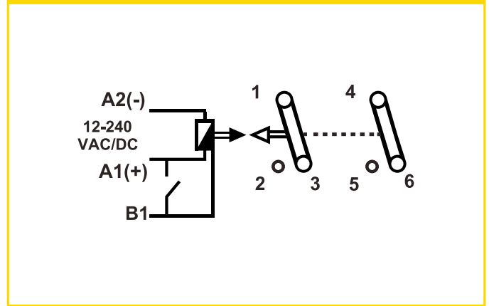
Connection Diagram
