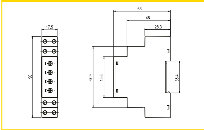
Dimensions (mm)(Type PK 25)
